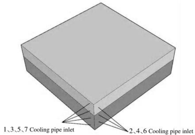
Figure 2. Model diagram of the outer surface of the pier cap.
