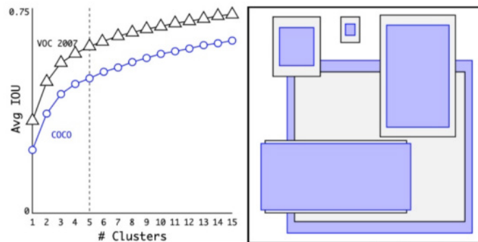
Fig3 Cluster analysis results
